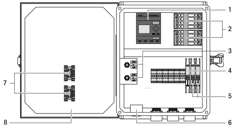
Model MVP-SSF1PTRO/DM panel shown
