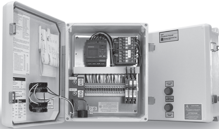
Easy to set, accurate, and surprisingly affordable, the MVP brings intelligent control technology to the water and wastewater handling industries. (Model MVP-SSF1PTRO/DM panel shown.)
