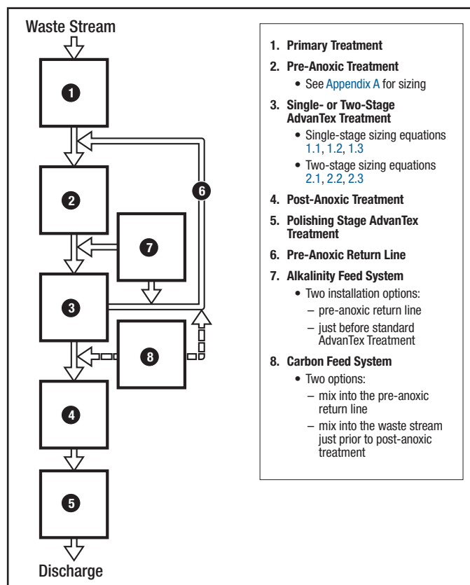
Figure 6. Treatment Diagram for Advanced Removal of Nitrogen
