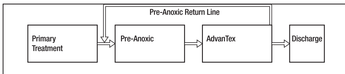
Figure D1. Treatment Configuration for Organic Constituents
