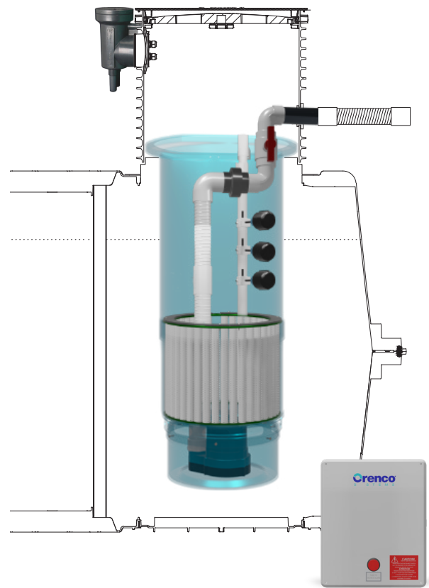
Effluent Pumping System: Simplex LHV inside Infiltrator™ CM-1060 Tank
