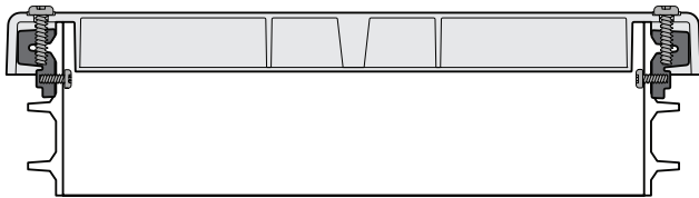
FL12GTU cap installed with bolt catches and cap screws (cross-sectional view)
