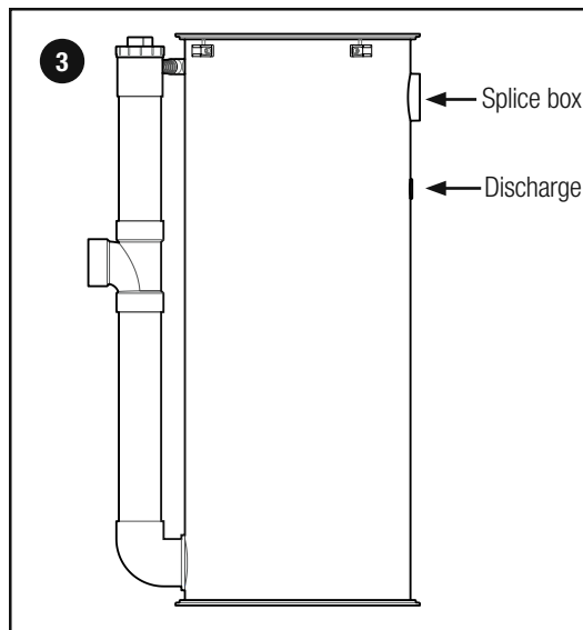
Install the grommets and adapters, if necessary.
