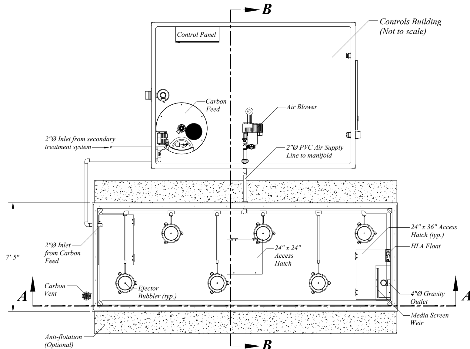
OmniMax-D-0821 Plan View Scale: 1" = 4'-0"
