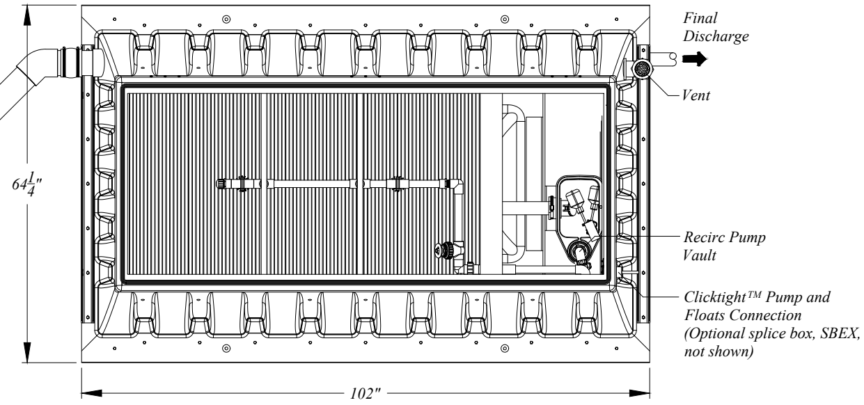
AX20 Recirc. Tank - Top View
