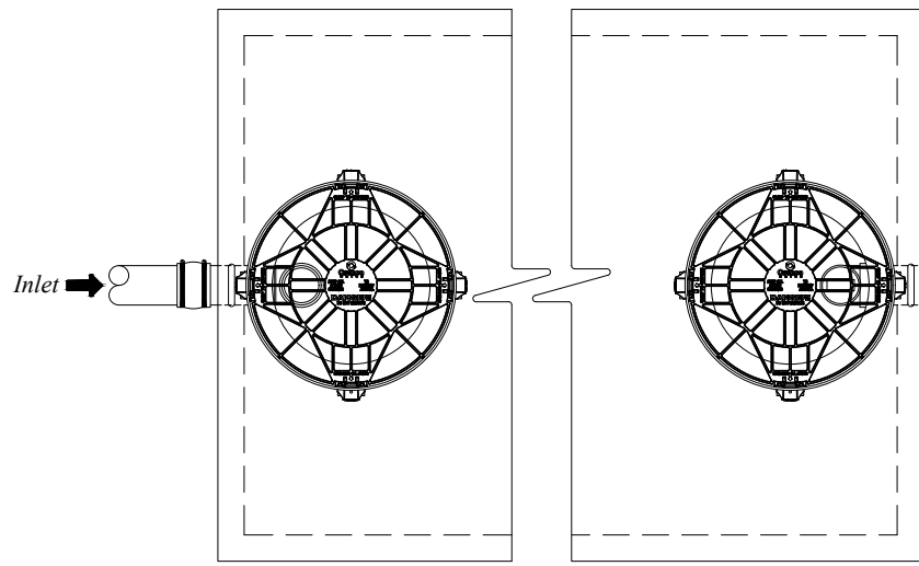
1000 gal. Primary Tank - Top View
