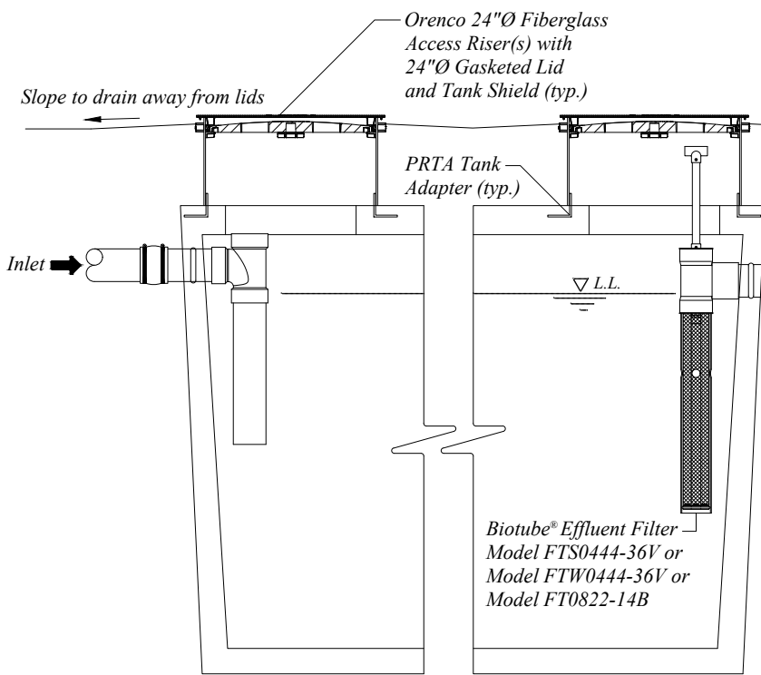
1000 gal. Primary Tank - Side View
