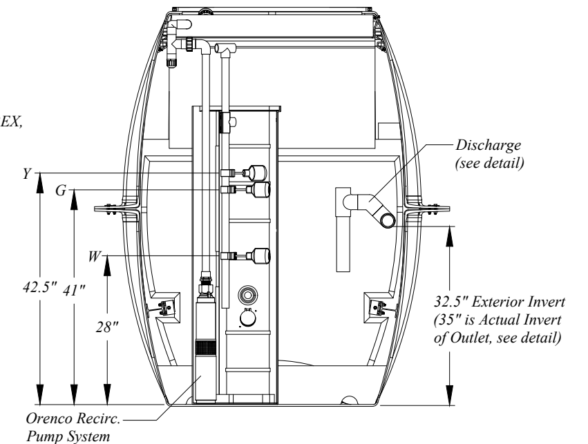
Discharge Chamber - End View
