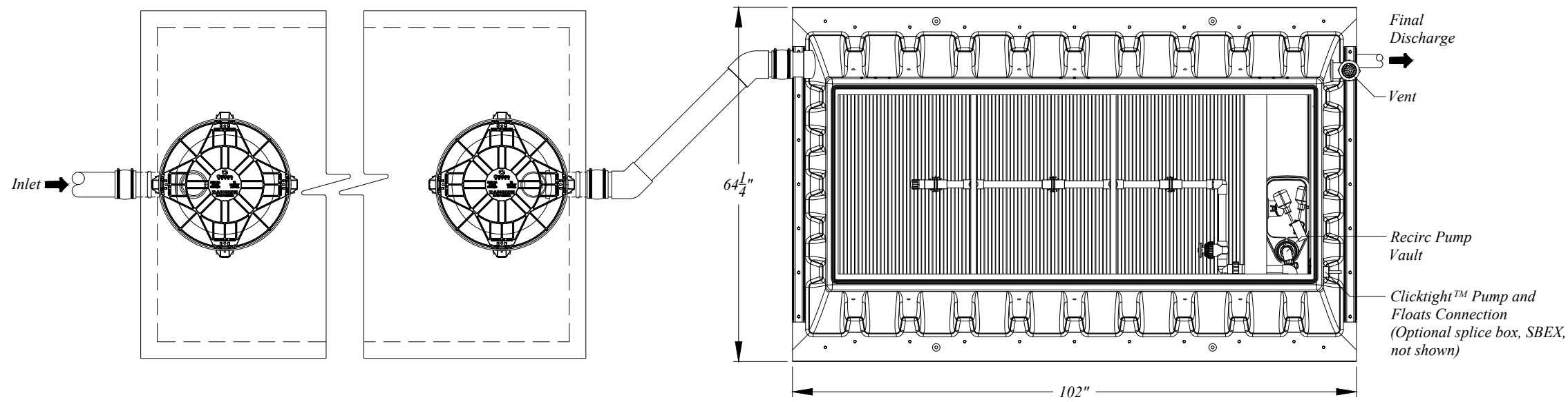
* Primary Tank - Top View
