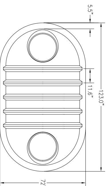
Top View
