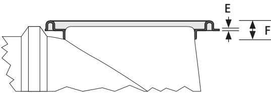
FRTA30-FRP, cross-sectional side view, as installed
