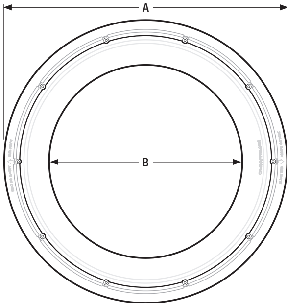
OR-SNAPPAR-2400, top view
