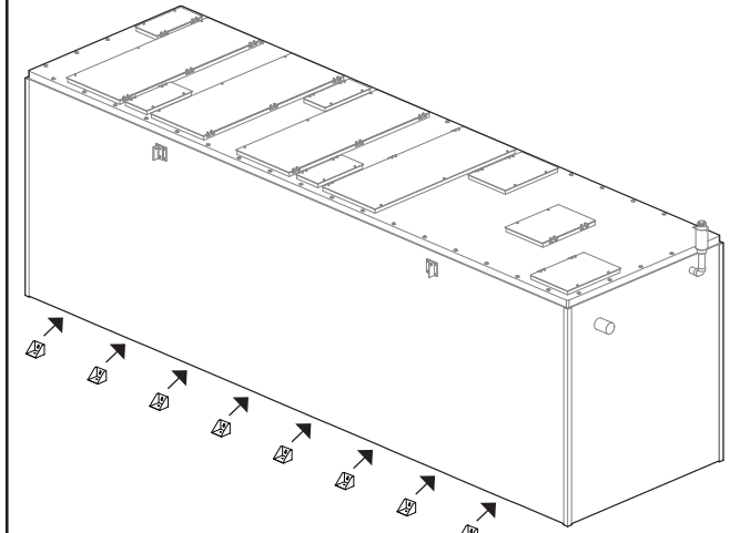
Anchoring bracket installation locations, one side
