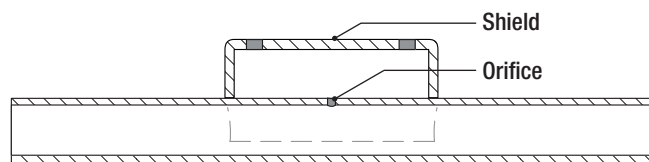
Standard configuration, side cutaway view
