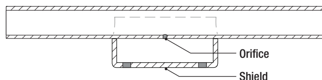
Cold weather configuration, side cutaway view
