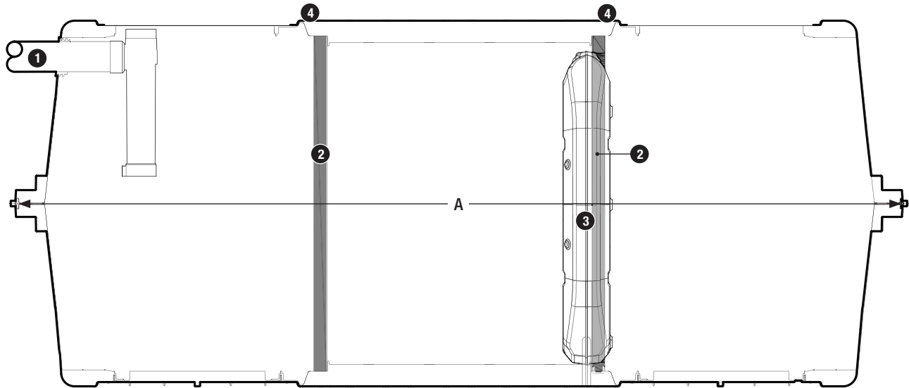
Infiltrator PS-1060 tank, side sectional view,
