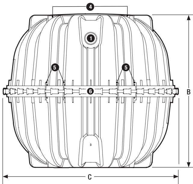
Infiltrator PS-1060 tank, end view
