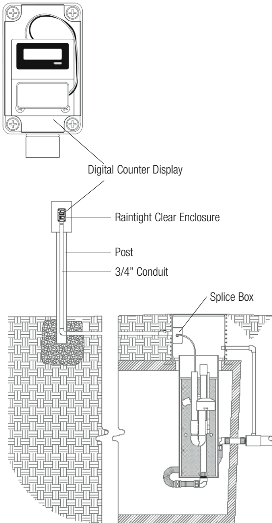
Side view of dosing siphon with digital dose counter.
